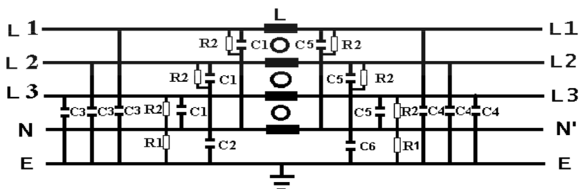
AC circuit (One-stage)
