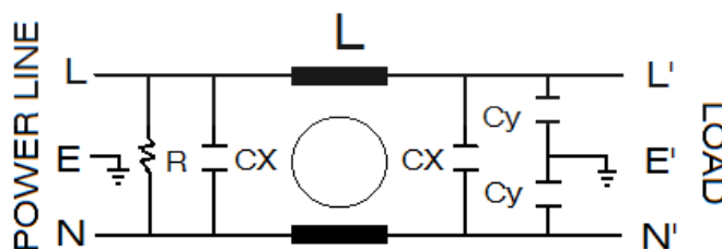
AC circuit (single-stage)
